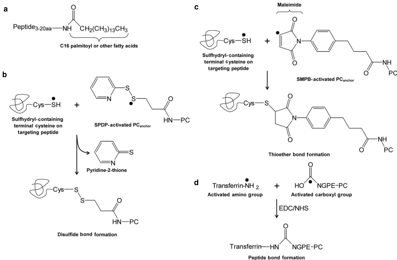
Figure 4. Some common chemistry for conjugating targeting ligands to lipid anchors. (a) For short peptides containing about 3–20 amino acids, a 16-carbon chain palmitoyl or other fatty acid chains may be attached to the protein through a lysine, cysteine (Cys), or glycine residue on either the N-terminal or C-terminal end of the protein sequence. (b) A sulfhydryl-containing terminal Cys on a targeting peptide ligand can be coupled to succinimidyl 3-(2-pyridyldithio)propionate-activated phosphatidylcholine (PC) lipid anchors, forming disulfide bond linkages. (c) A sulfhydryl-containing terminal Cys on a targeting peptide ligand can be coupled to succinimidyl-4-(p-maleimidophenyl) butyrate-activated PC lipid anchors, forming stable thioether linkages. (d) An activated amino group on a targeting peptide ligand (e.g., transferrin) can be coupled to an activated carboxyl group on a PC lipid anchor [e.g., N-glutaryl phosphatidylethanolamine (NGPE)-PC] through a carbodiimide reaction with ethyl(dimethylaminopropyl) carbodiimide/N-hydroxysuccinimide (EDC/NHS), forming peptide bond linkages. Addition of NHS to EDC reactions increases efficiency. The black dot indicates atoms that form the bond of interest.
