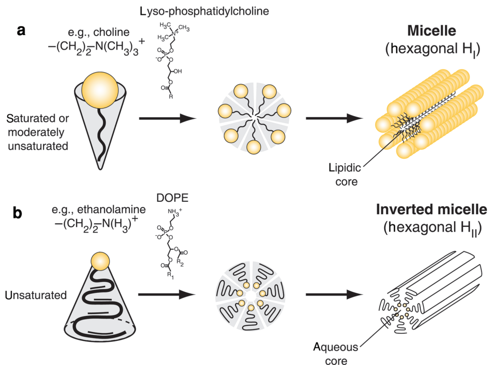
Figure 2. A schematic presentation of lipids and derivatives that form micelles and inverted micelles. (a) Lipidic micelles (hexagonal H_I ) are formed because of a large hydrophilic head group, such as a lyso-phosphatidylcholine with a choline head group and a saturated fatty acid. They form stable molecular aggregates that resemble sheets of tubes with an internal lipidic core. (b) Inverted micelles (hexagonal H_{II} ) are formed because of phospholipid with a neutral and small head group, such as phosphatidylethanolamine, with unsaturated fatty acyl tails that tend to form inverted cone structures in solution (e.g., 1,2-dioleoyl-sn-glycero-3-phosphoethanolamine or DOPE). They form stable molecular aggregates that resemble sheets of tubes with an internal aqueous space.
