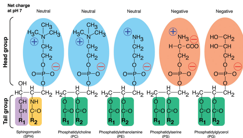
Figure 1. A schematic presentation of commonly used phospholipids. Most of the commonly used lipids are presented with hydrophobic R_1 and R_2 fatty acyl tail groups and a hydrophilic head group carrying a net charge at neutral pH 7. The head group determines the charge of a phospholipid, whereas the lipid tail group contributes no charge. The lipids with head groups (oval shape shaded area) for sphingomyelin (SPH), phosphatidylcholine, and phosphatidylethanolamine exhibit neutral net charge. Phosphatidylserine and phosphatidylglycerol carry a negative net charge at neutral pH 7. The tail groups ( R_1 and R_2 ) for each phospholipid can have various lengths (typically C14–C18) and degrees of saturation. SPH contains a sphingoid base backbone (unshaded) and the other four phospholipids contain a glycerol backbone (unshaded). In addition, R_1 of SPH is a C15-saturated carbon chain and R_2 is a fatty acid residue connected to the sphingoid base backbone through an amide functional group. The fatty acid residues for the other four phospholipids are attached to the glycerol backbone via an ester functional group. The detailed effects on the physical properties of phospholipids because of charge and variation in R_1 and R_2 are described in Table 3.
